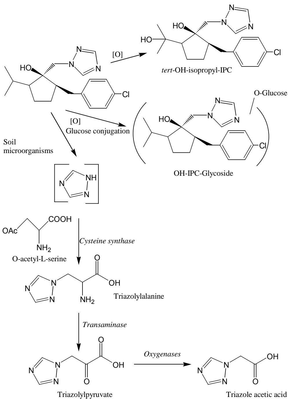
Proposed metabolic pathway for the metabolism of ipconazole in wheat
