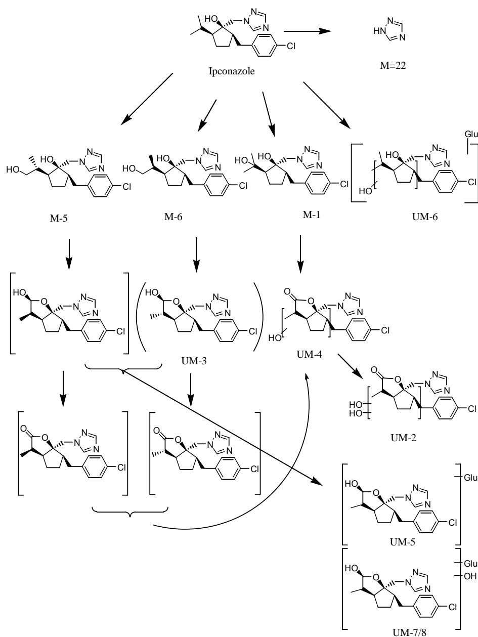
The proposed biotransformation pathway for ipconazole in goats
