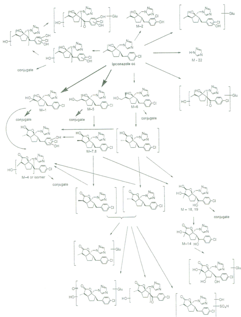
The proposed biotransformation pathway for ipconazole in rats
